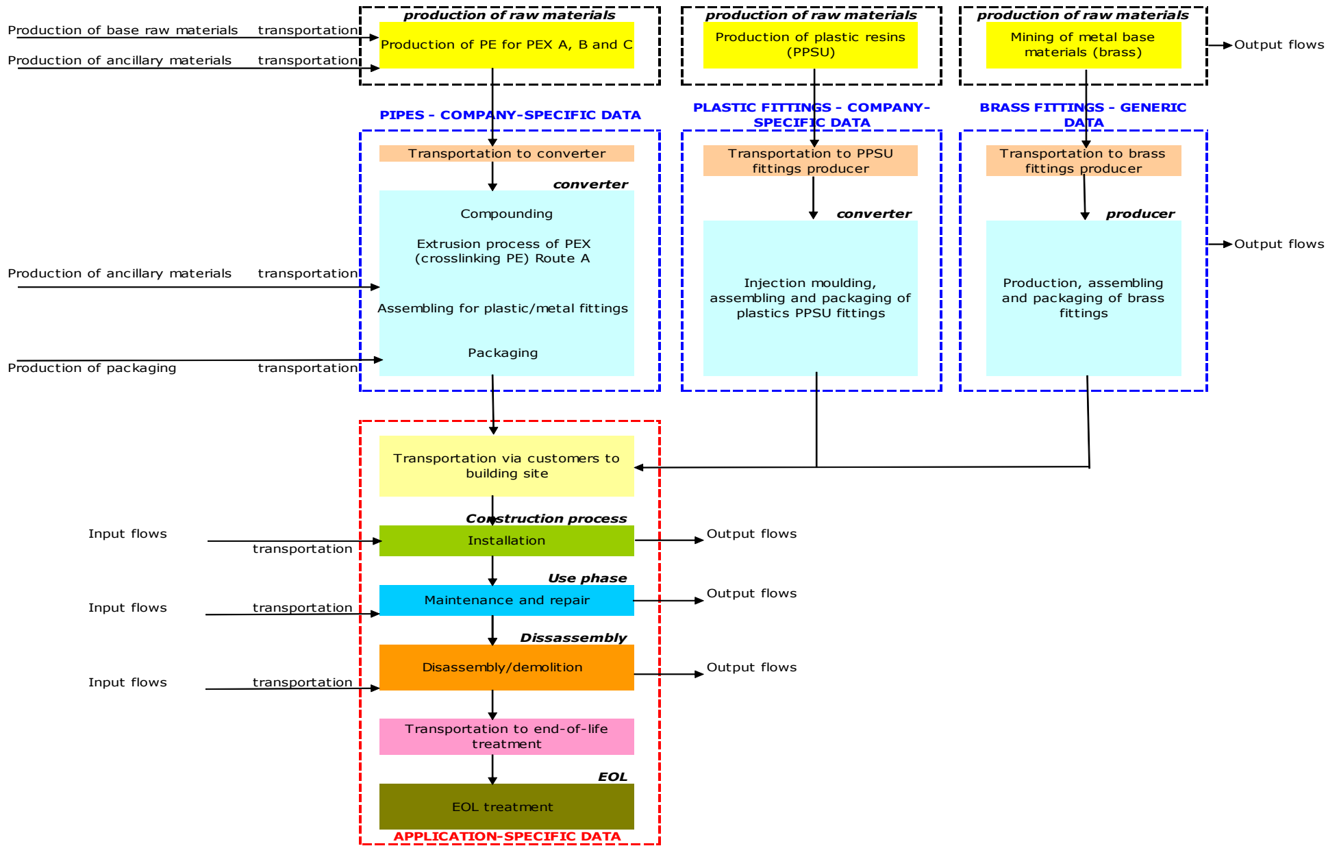
Life cycle flow chart of the PEX Hot & Cold water pipe system (Buildings)
