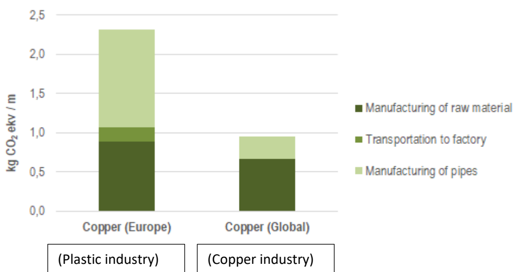
Figure 1. Carbon footprint of a metre of copper pipe according to calculations by the plastic and copper industries. In the bar for the plastic industry, the sensitivity analysis (white line) shows the change in the recycling rate of copper raw material 26 -> 90% and the copper industry bar shows the impact if mining activities are excluded from the impacts of raw material production. The latter of these sensitivity analyses was carried out because it remained somewhat unclear to what extent mining was involved in the assessment of the plastic industry.
