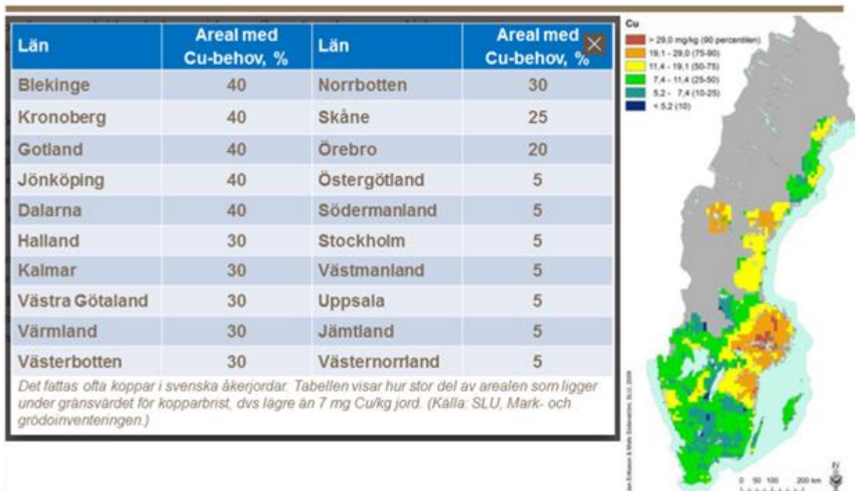
Figure 2. Copper concentrations and need for copper on Swedish cultivated land (SLU 2020, table by YARA). Fertilisation with sludge containing copper is not recommended in Sweden if copper content in soil is more than 40 mg/kg. This kind of soils are 3.7 % of field area in Sweden.
