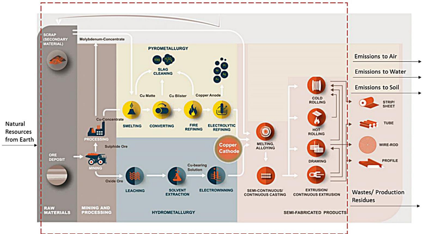
Figure 1. Phases of manufacturing copper products (ECI 2016).
