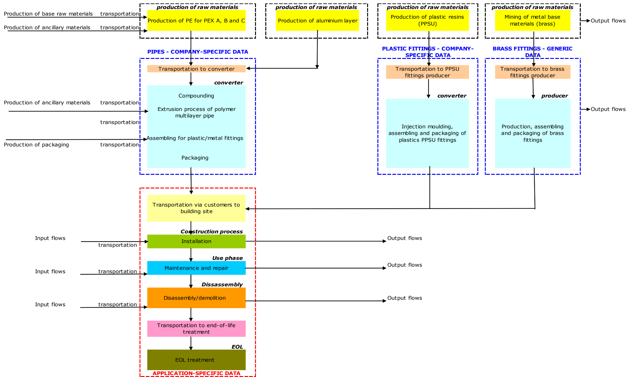
Life cycle flow chart of the polymer multilayer hot & cold water pipe system (Buildings)
