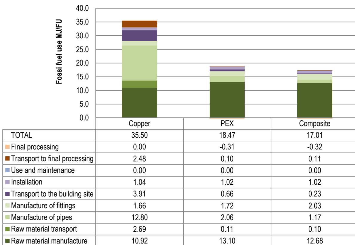
Figure 3. The fossil fuel use (MJ) resulting from different pipe materials per functional unit according to assessments by the plastic industry.
