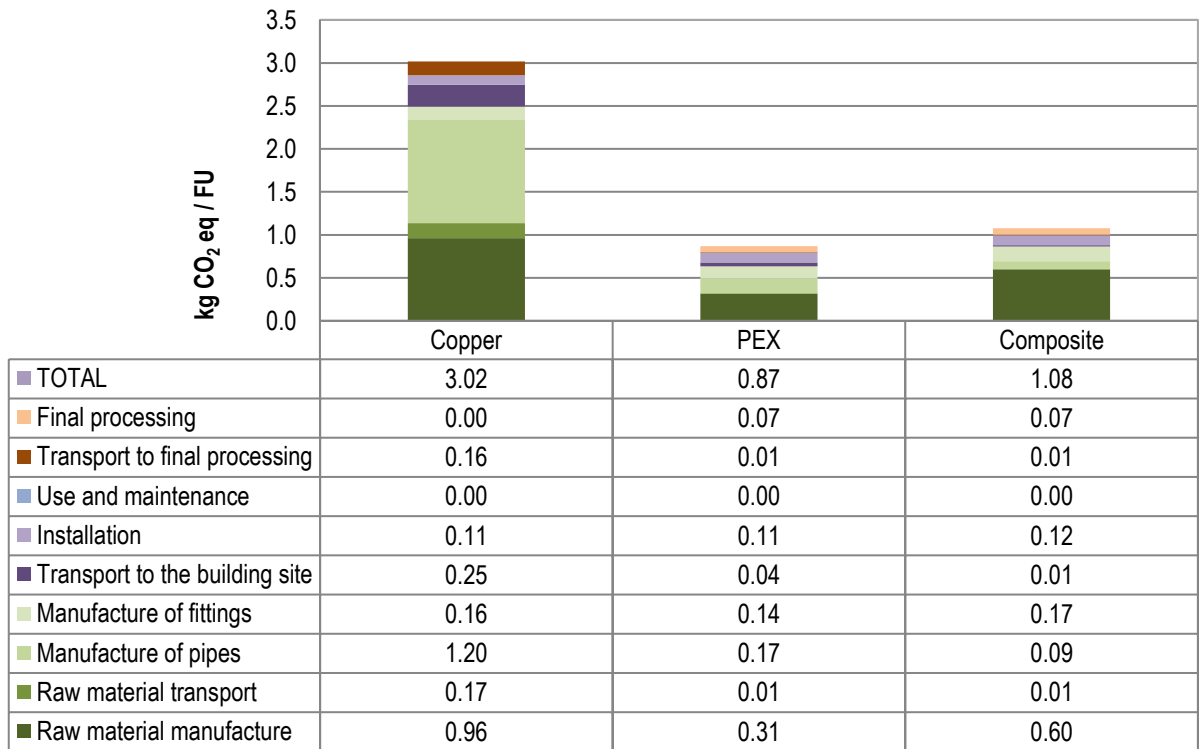
Figure 2. The climate change impacts of different pipe materials per functional unit (kg CO 2 equivalent), according to assessments by the plastic industry.
